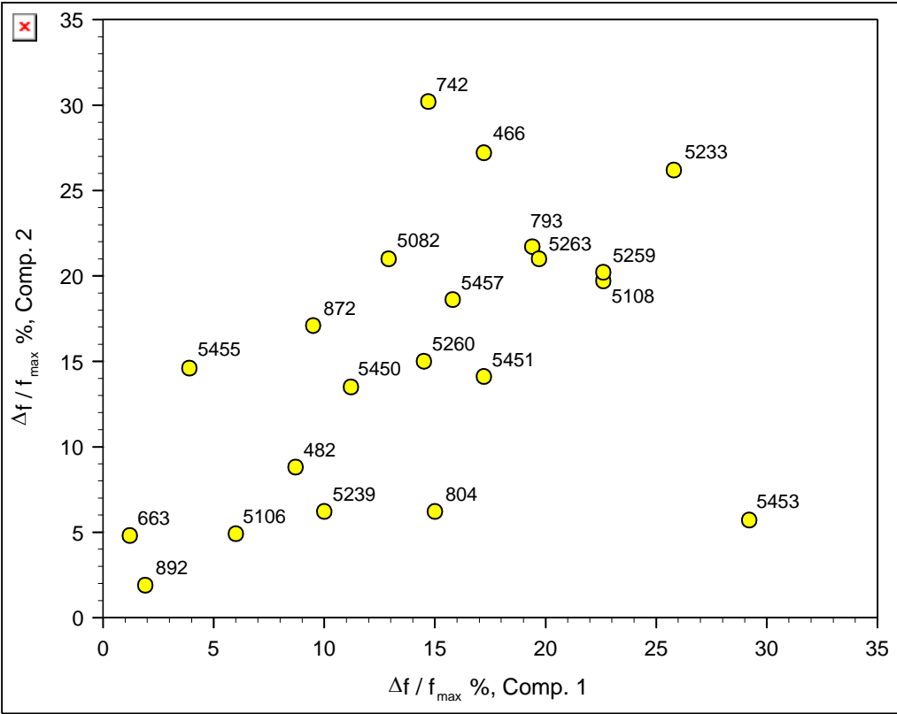
Figure 3 Observed changes in system frequency for 21 buildings.
