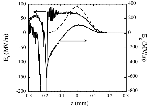
Figure 2: Transverse ( E_r , thin line, left hand side scale) and longitudinal ( E_z , thick line, right hand side scale) wake fields excited by the beam (shown by the dotted line) with parameters given in Table 1 in a plasma with n_p = 1.5 \cdot 10^{14} \text{ cm}^{-3} .
